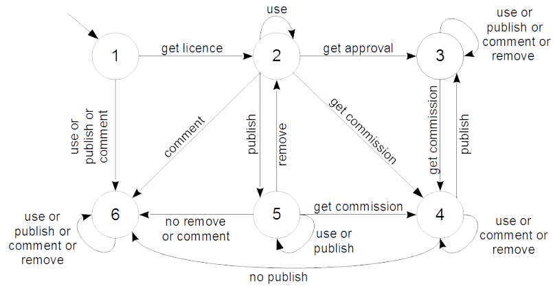
Fig. 1. State machine of the licensing contractual clauses.
